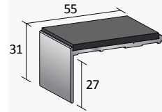
SF11 - single channel flat
