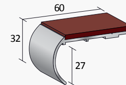
HF31 - single channel bullnose
