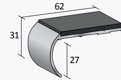
SF31 - single channel bullnose
