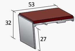
HF51 - single channel raked
