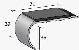
SF161 - single channel bullnose - ramp back
