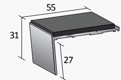
SF51 - single channel raked
